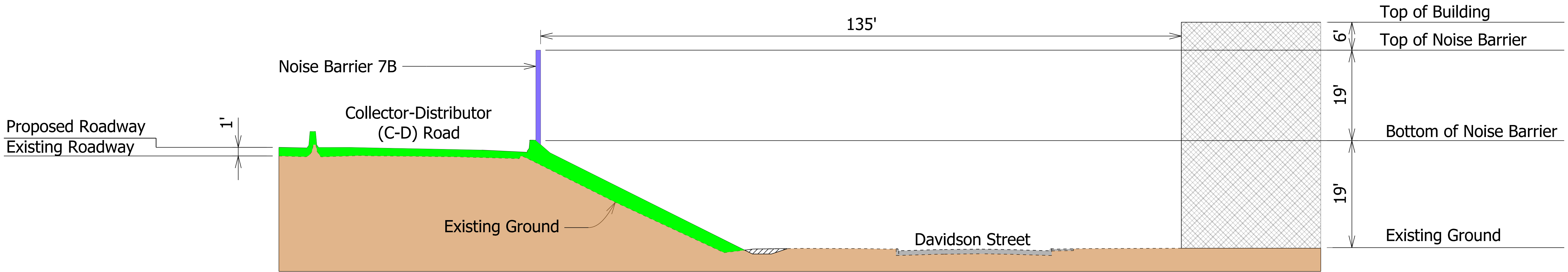
SECTION VIEW "A-A"
