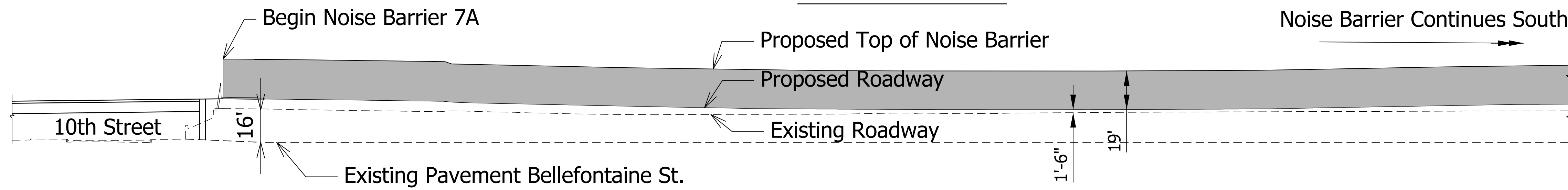
ELEVATION VIEW FROM BELLEFONTAINE ST.
