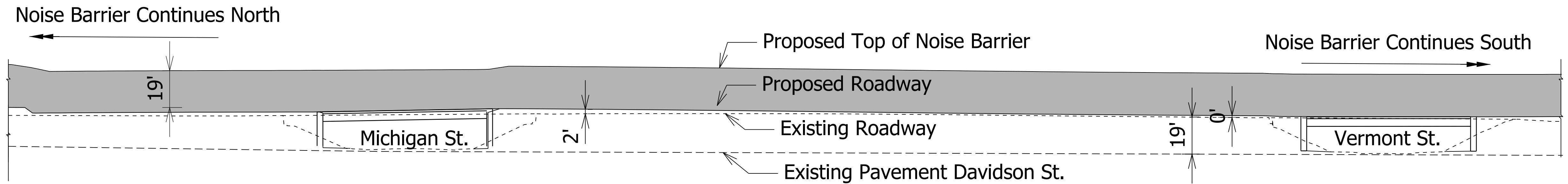
ELEVATION VIEW FROM DAVIDSON STREET
