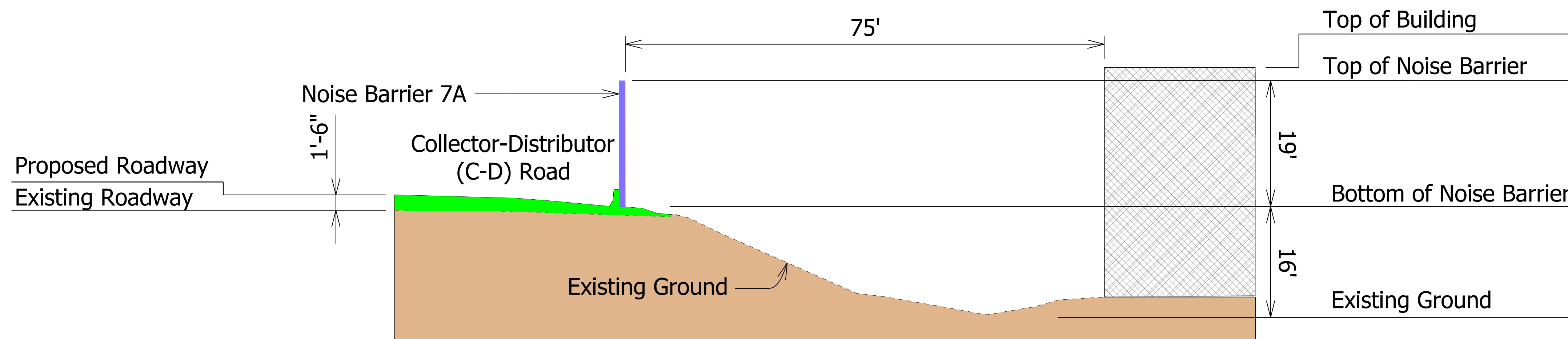
SECTION VIEW "A-A"
