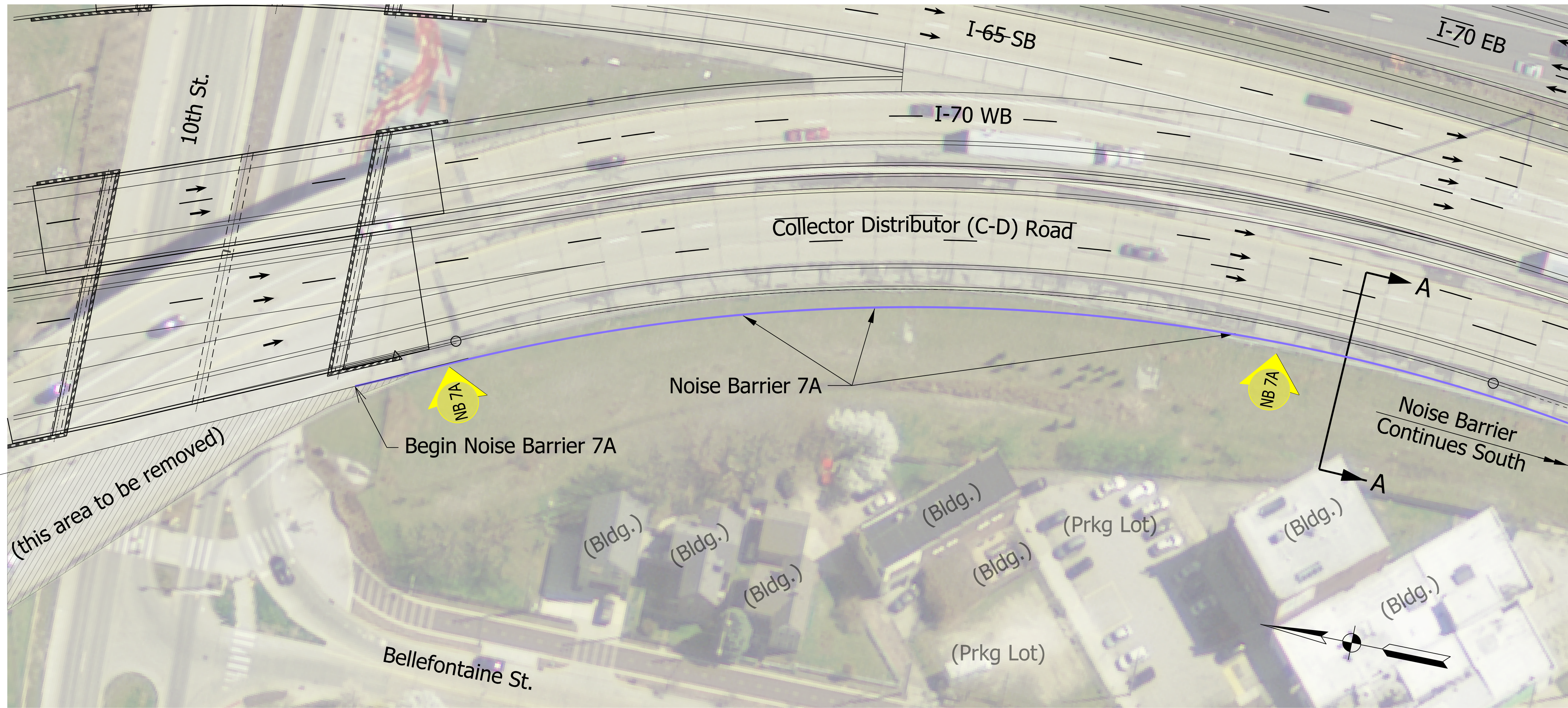
PLAN VIEW
