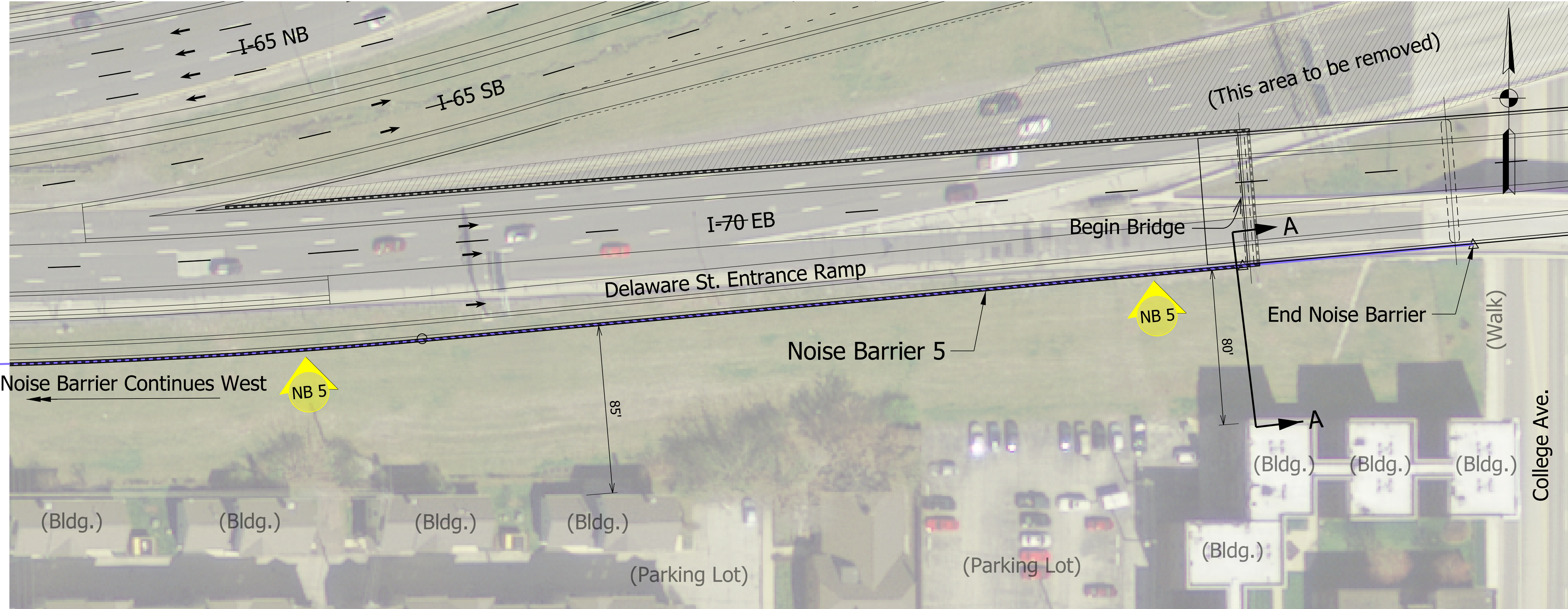
PLAN VIEW
