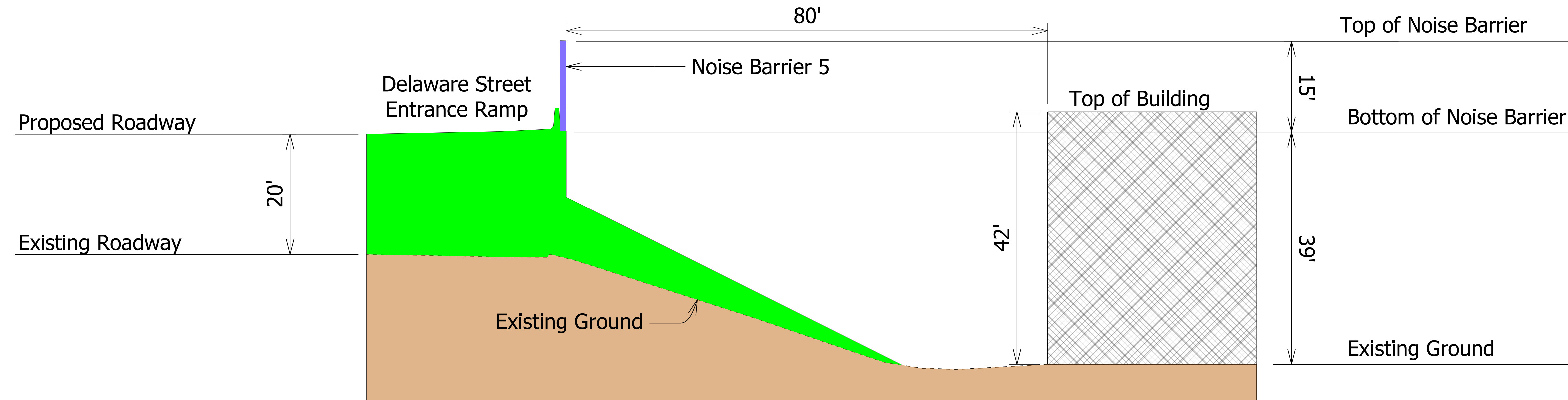
SECTION VIEW "A-A"
