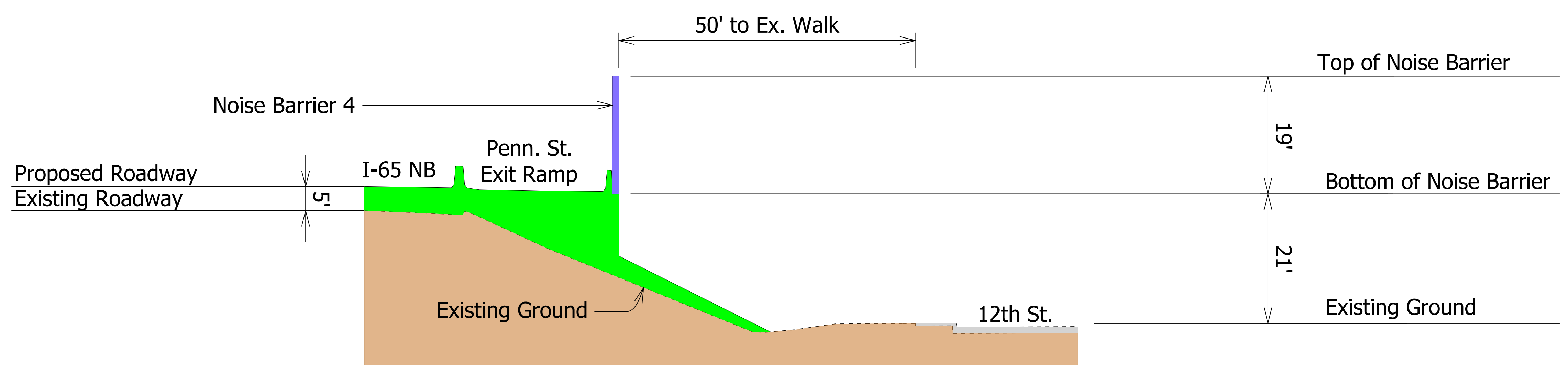
SECTION VIEW "A-A"
